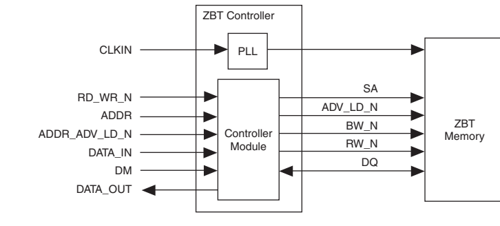
Figure 2. ZBT Controller System-Level Diagram
