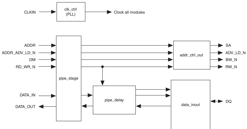
Figure 3. ZBT Controller Low Level Modules
